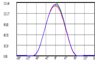
Light Distribution Curve:(cd)
