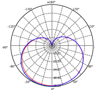
Light Distribution Curve:(cd)
